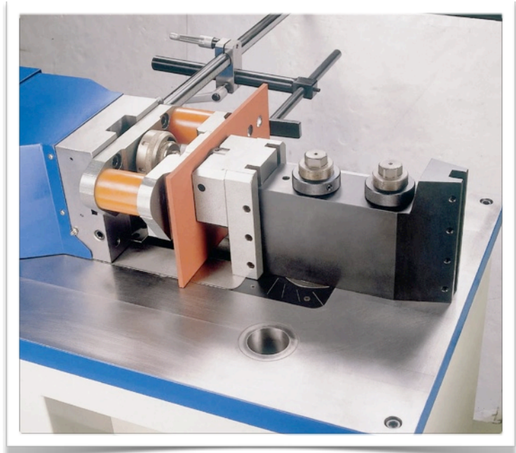
Punching Tool
