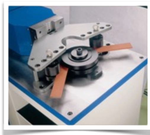
Flat Bar Bending Tool
