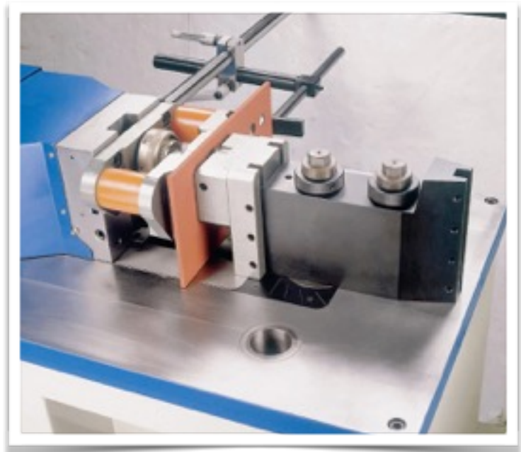
Punching Tool
