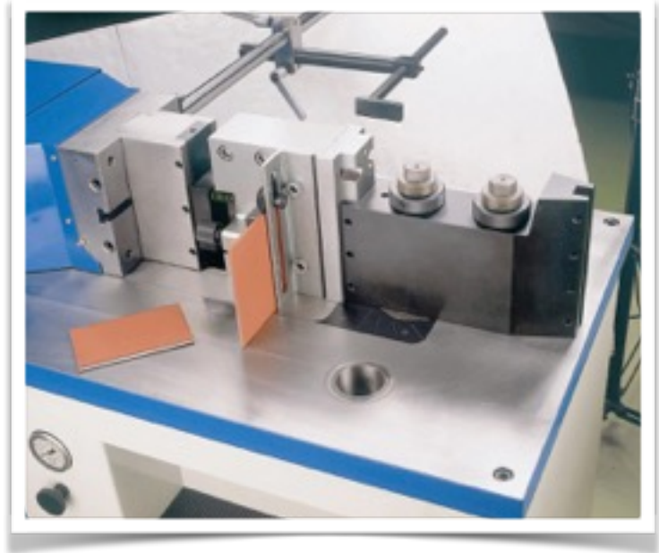
Flat Bar Shearing Tool
